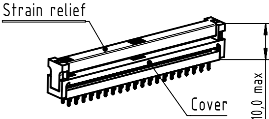
Assembled cover with strain relief
